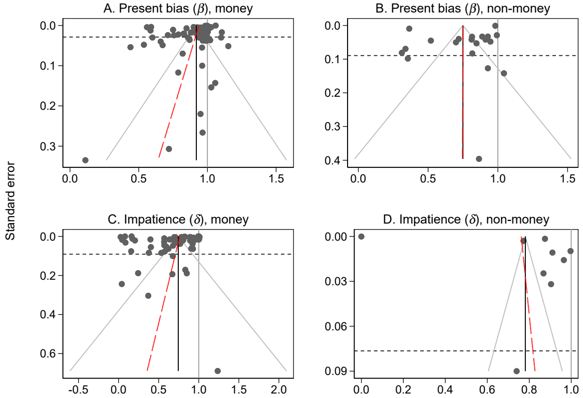
Figure 2: Funnel plots of \beta and \delta estimates
